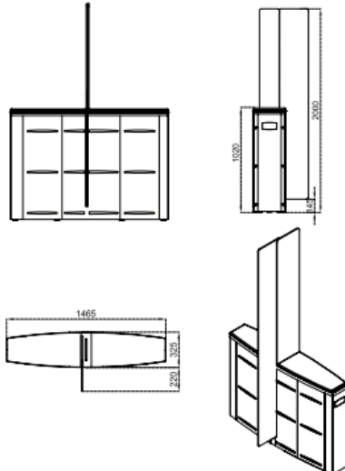
SG 55 T-S Glass Wing Height : 2000 mm
